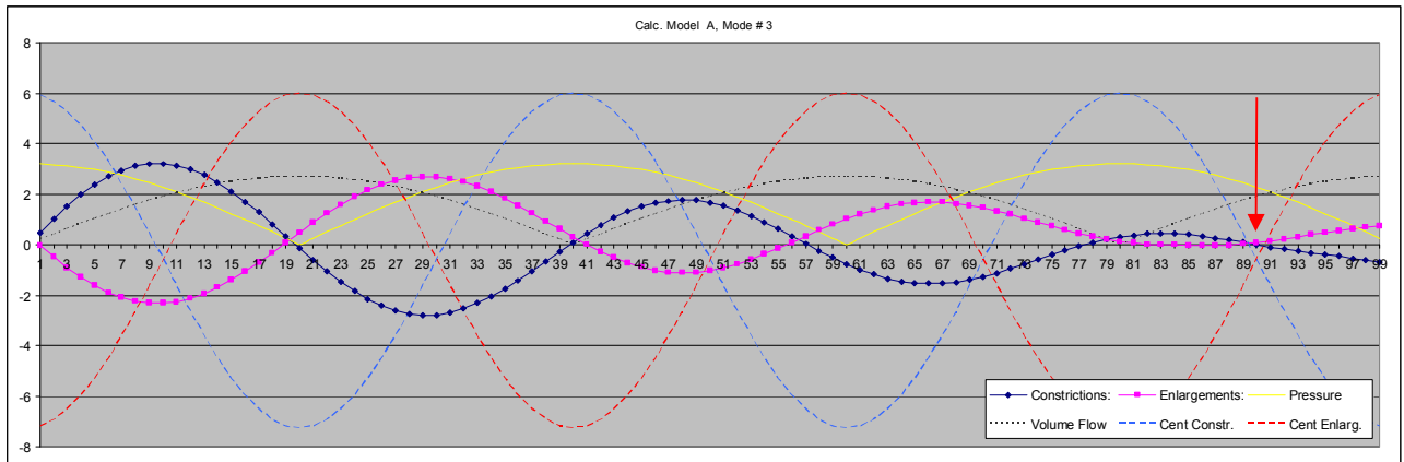
Cylinder L=1000mm, Bore =11mm, Constrictions =10mm, Enlargements =12,1mm, Pert. Length = 20mm. y-Axis: Magnitudes = % Change |Z|in, Pitch: Cent Deviation from the unperturbated closed-open Tube. x-Axis: Center-Position of each single local Perturbation applied, in % of tube length (Example Mode = #3)
