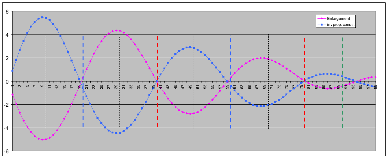
|Z|in Magnitude Change %, result of OpenWind Simulations with same perturbations as repeatedly measured. blue dotted lines: expected Position of Pressure Nodes, red dotted lines: Pressure Antinode Positions
