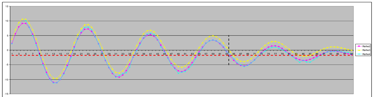
Mode #6, turquoise=measured value of magnitude change, pink=modeling result, yellow=without offset dn Mode #6, last 4/4 WL starts at 63,36% tubelength
