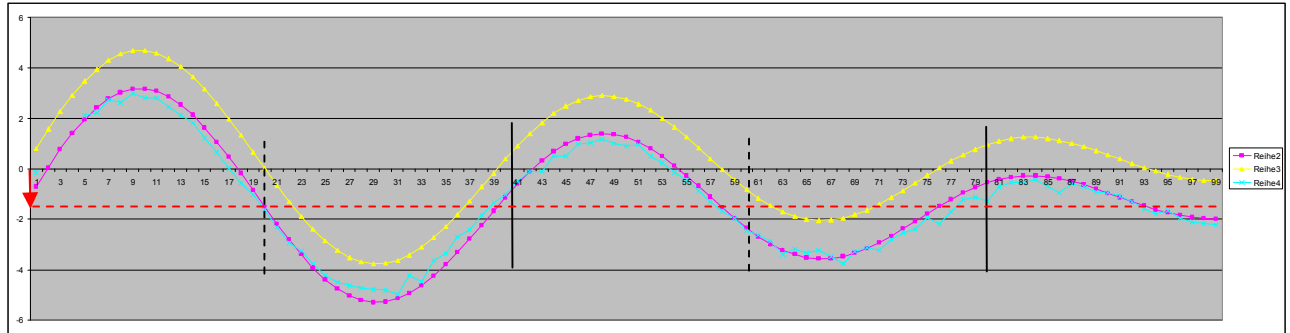
Mode #3, turquoise=measured value of magnitude change, pink=modeling result, yellow=without offset dn Mode #3, last 4/4 WL starts at 20% tubelength = a pressure node, (dotted lines);
